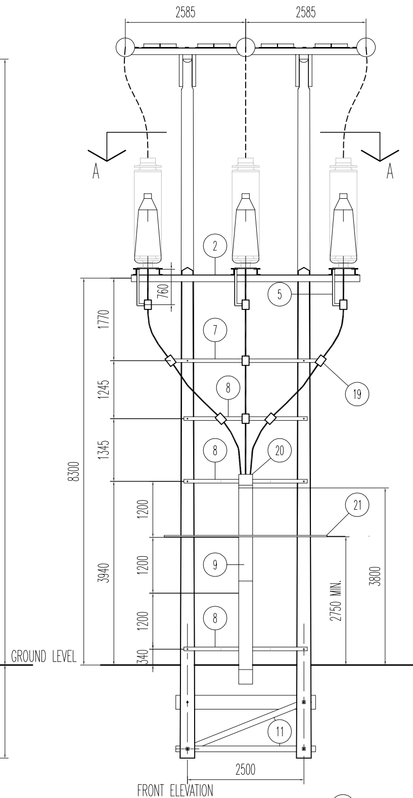
PART DETAIL OF FRONT ELEVATION
